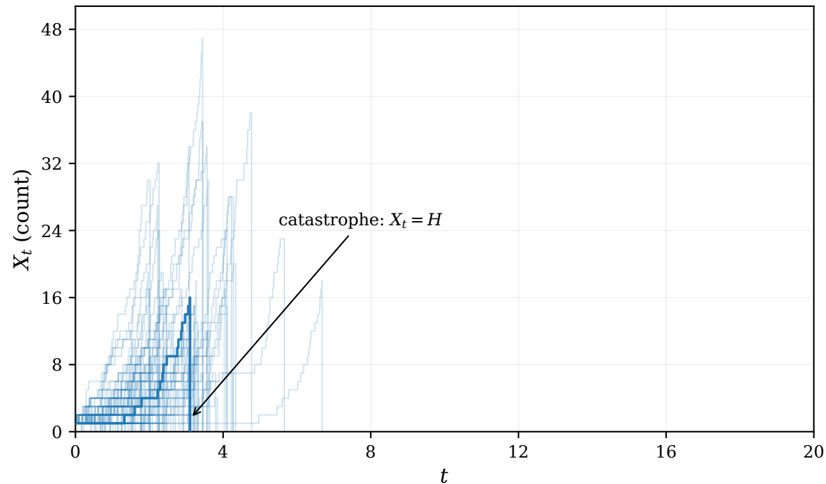
100 Gillespie realisations of X_t
